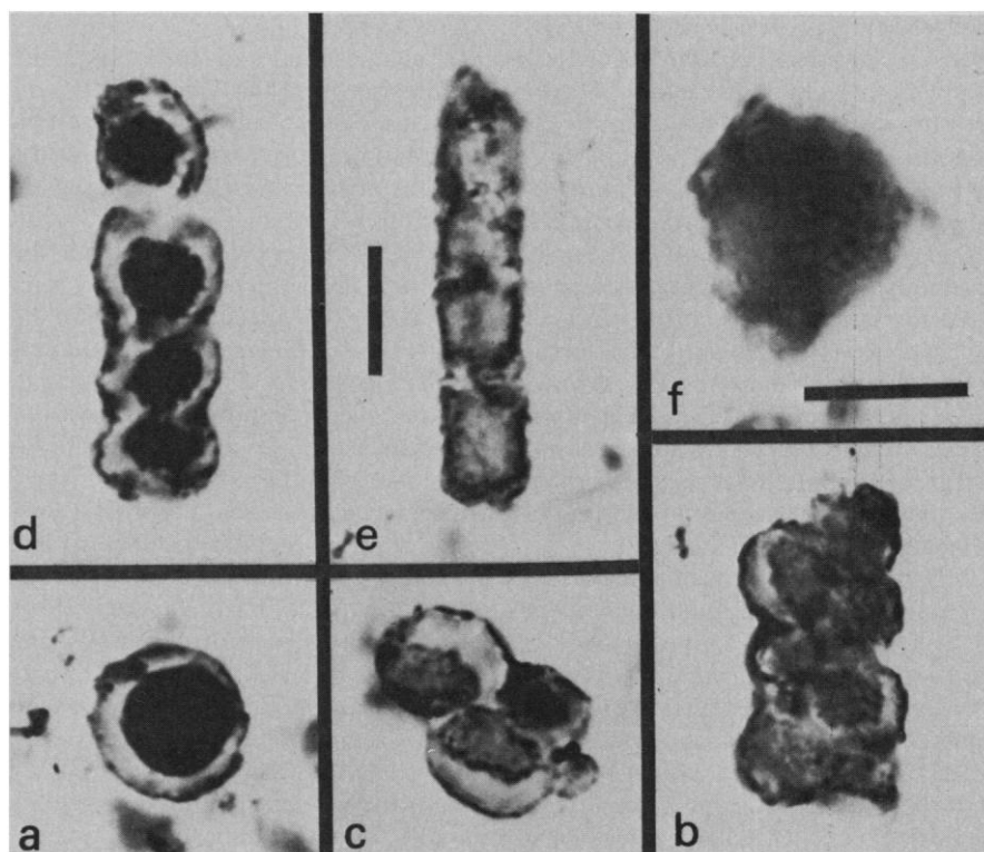
Fig. 1. (a) Spherical cell with internal structure of organic material. (b) Cluster of cells with internal granular structures. (c) Cluster of cells with internal granular structures and small budlike cell. (d) Filament of spherical cells with internal structures. (e) Cylindrical tube with crosswalls. (f) Bavlinella cf. faveolata . Scale bar in (e), which applies to (a) through (e), represents 10 \mu\text{m} ; bar in (f) also represents 10 \mu\text{m} .
