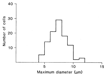
Fig. 2. Size frequency distribution of spherical cells ( N = 104 , \bar{X} = 7.2 \mu\text{m} ).
